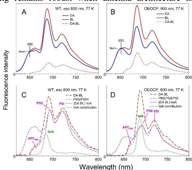
Figure 1. Blue-light induced difference spectra of WT and OEOCP Synechocystis 6803 at 77 K after PBS excitation (600 nm). (A–B) Fluorescence emission and difference spectra. (C–D) Spectral reconstructions showing contributions from IsiA, APC660, PSII, and PSI.
